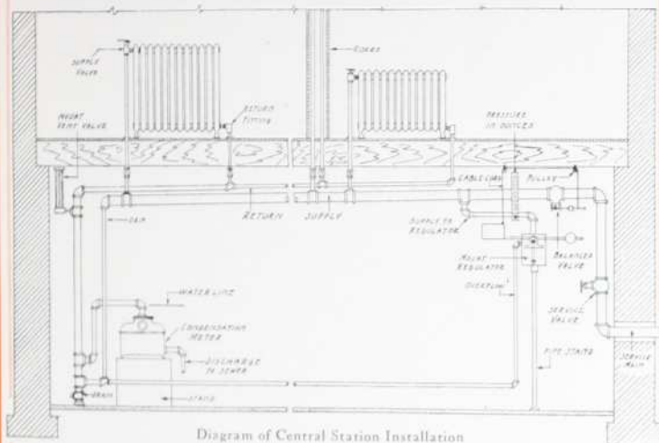
Diagram of Central Station Installation
